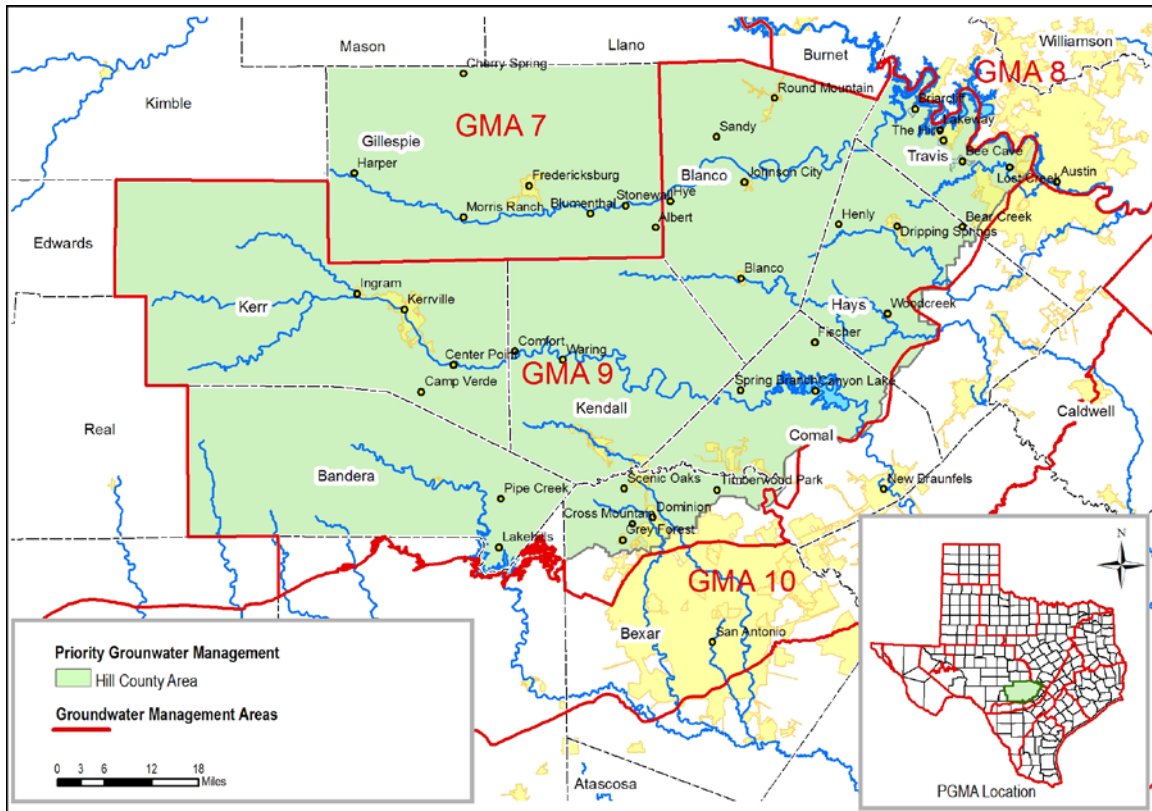
Figure II.-1 Location of Groundwater Management Area boundaries in the study area.
