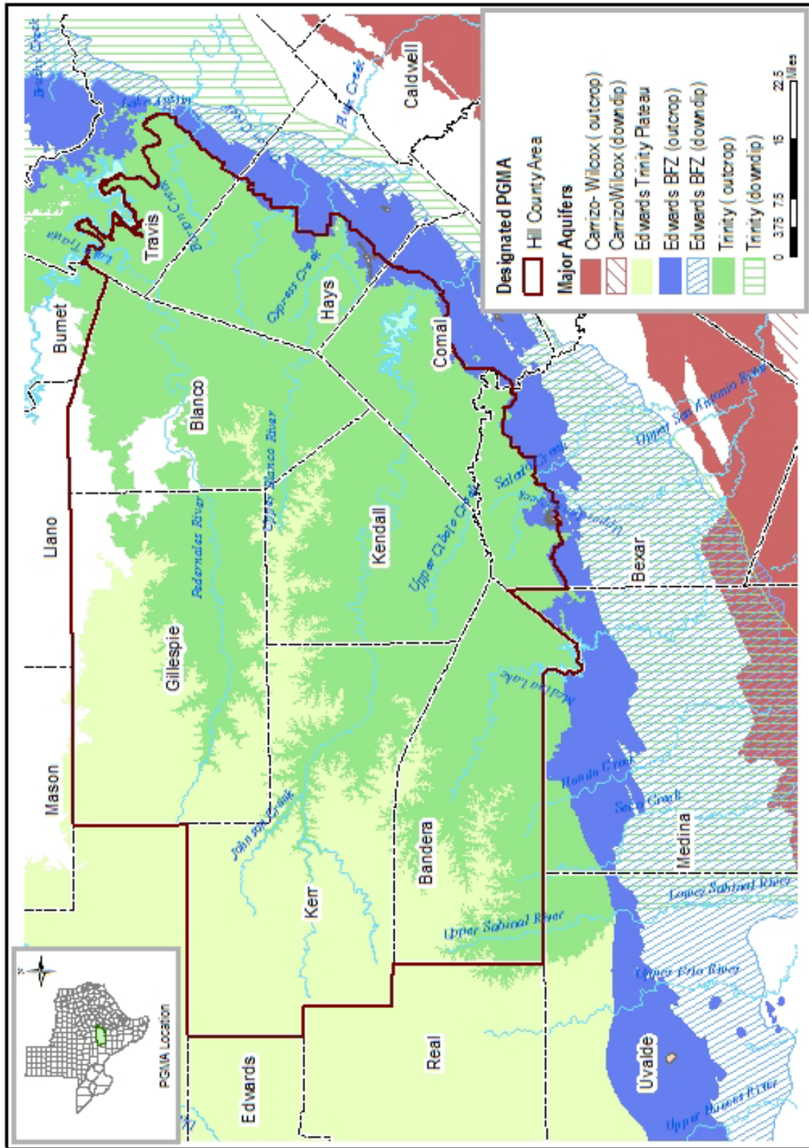
Figure 2. Major Aquifers in and Adjacent to the Hill Country PGMA
